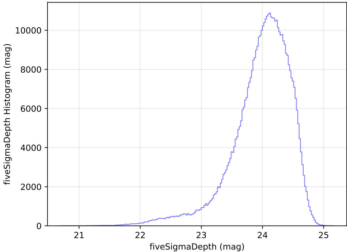
too_elab_r8_d3_griz_v3.4_10yrs r: fiveSigmaDepth Histogram
