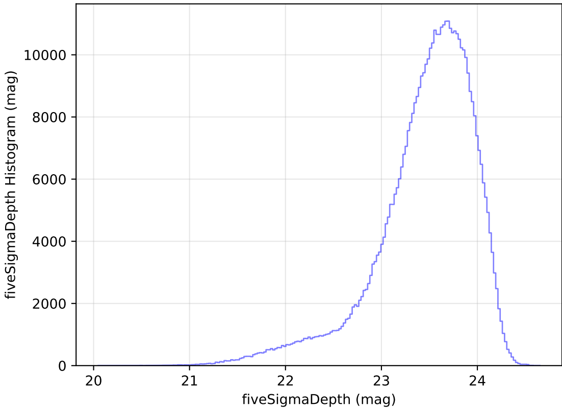
too_elab_r8_d3_griz_v3.4_10yrs i: fiveSigmaDepth Histogram
