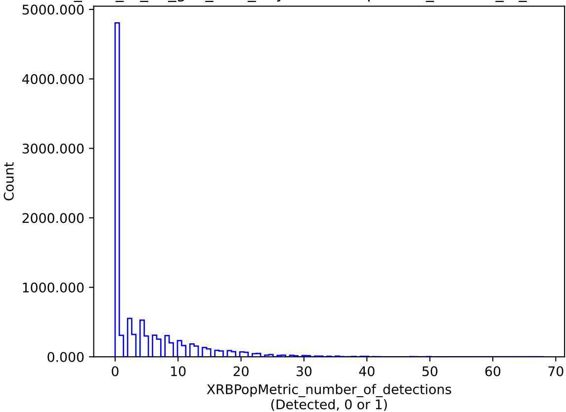
too_elab_r8_d3_griz_v3.4_10yrs : XRBPopMetric_number_of_detections
