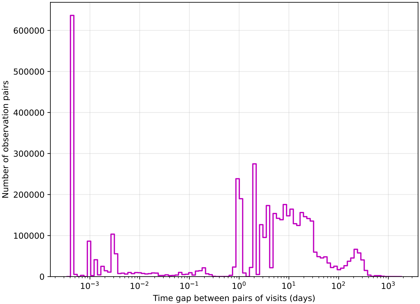
too_elab_r8_d3_griz_v3.4_10yrs z band: Tgaps observationStartMJD
