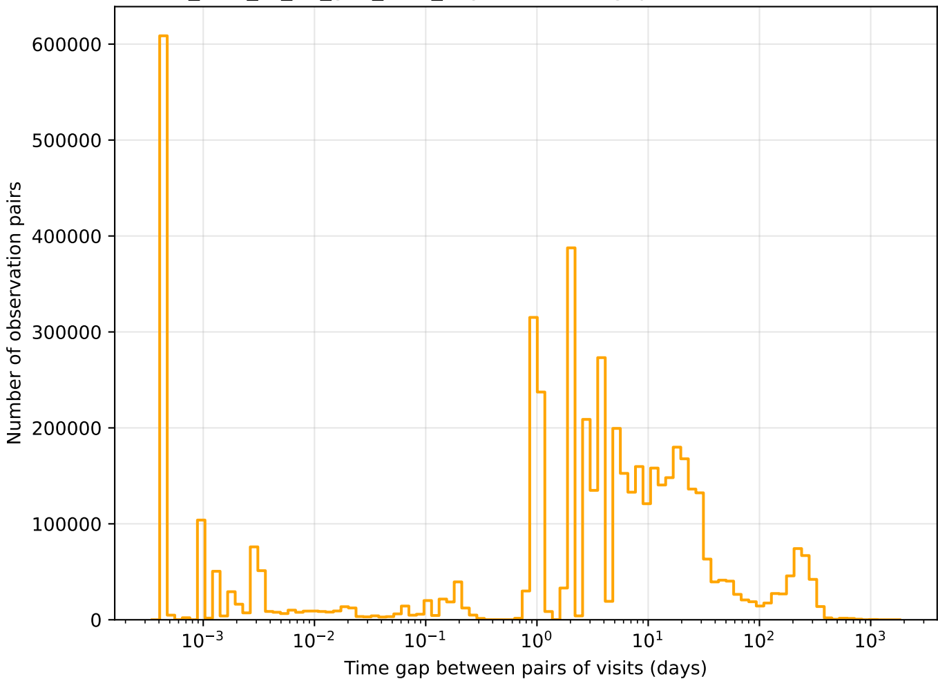
too_elab_r8_d3_griz_v3.4_10yrs r band: Tgaps observationStartMJD
