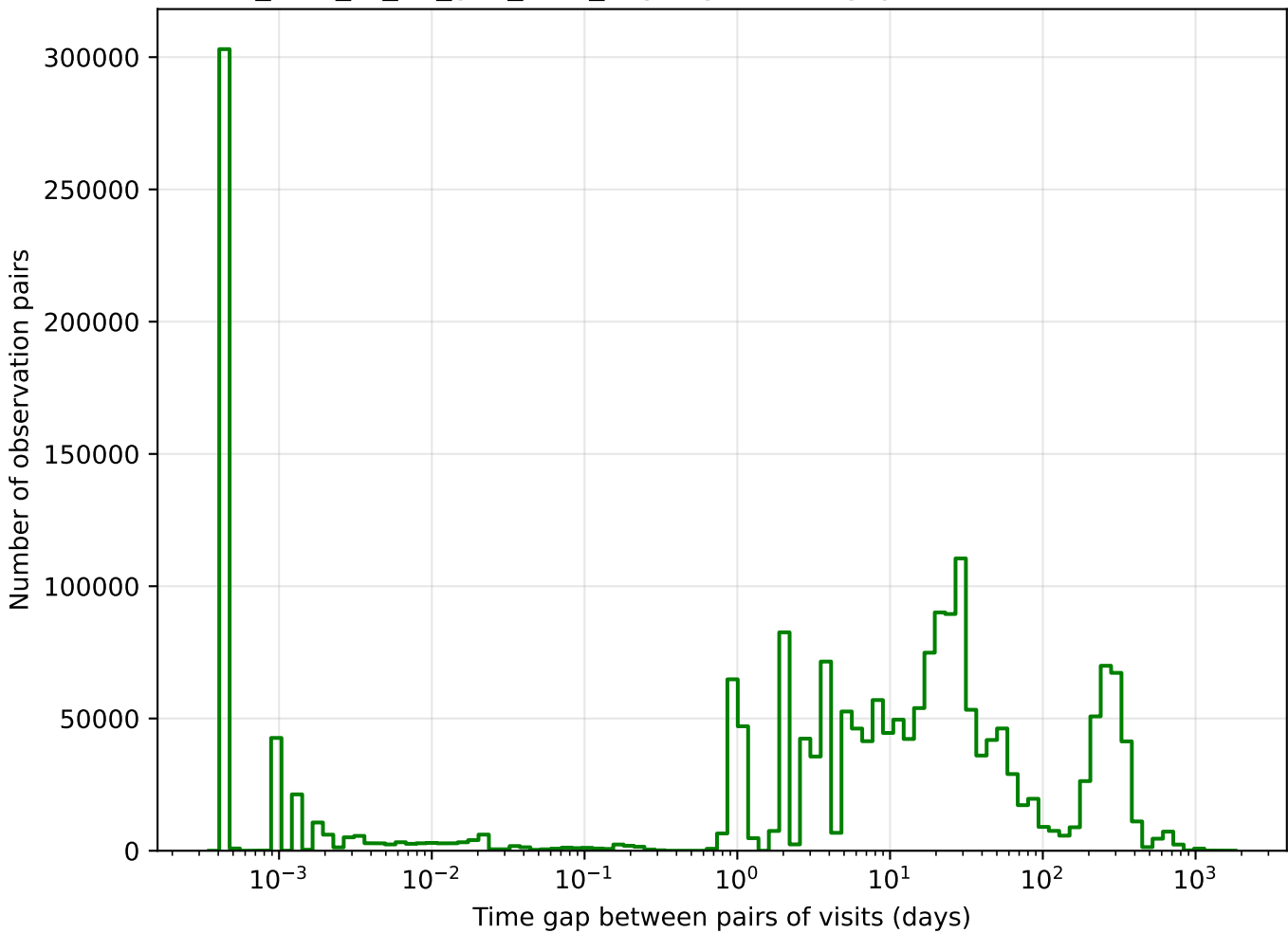
too_elab_r8_d3_griz_v3.4_10yrs g band: Tgaps observationStartMJD
