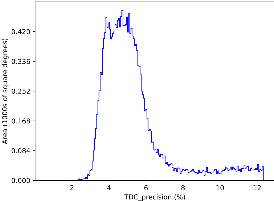
too_elab_r8_d3_griz_v3.4_10yrs : TDC_precision
