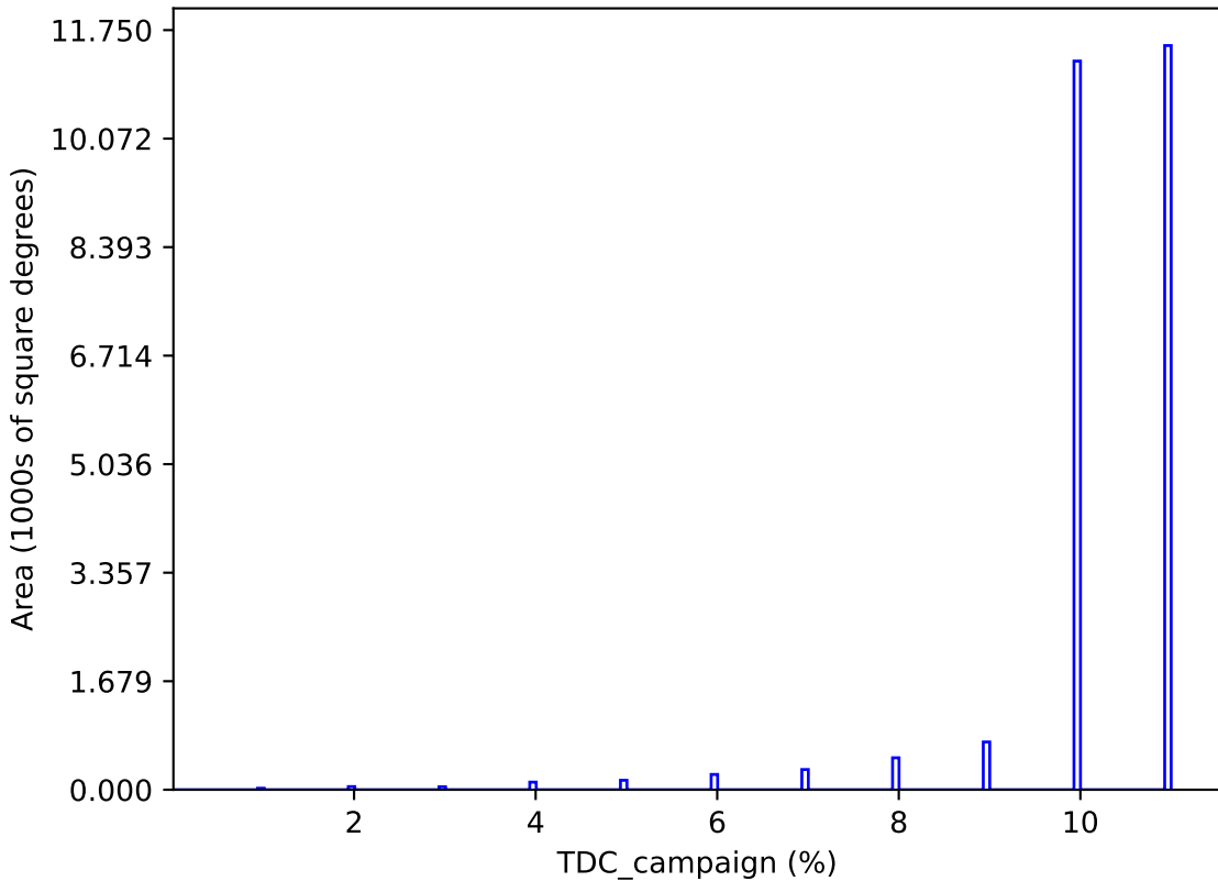
too_elab_r8_d3_griz_v3.4_10yrs : TDC_campaign
