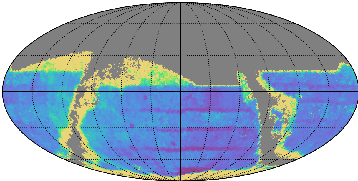
too_elab_r8_d3_griz_v3.4_10yrs : TDC_accuracy
