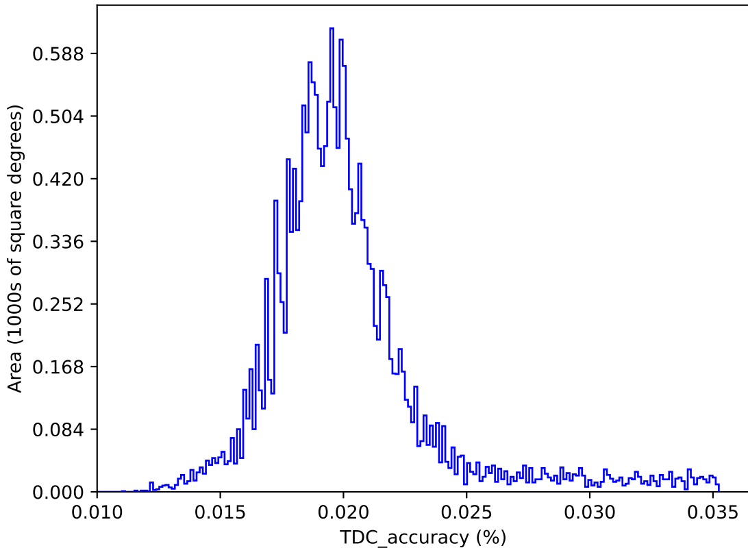
too_elab_r8_d3_griz_v3.4_10yrs : TDC_accuracy
