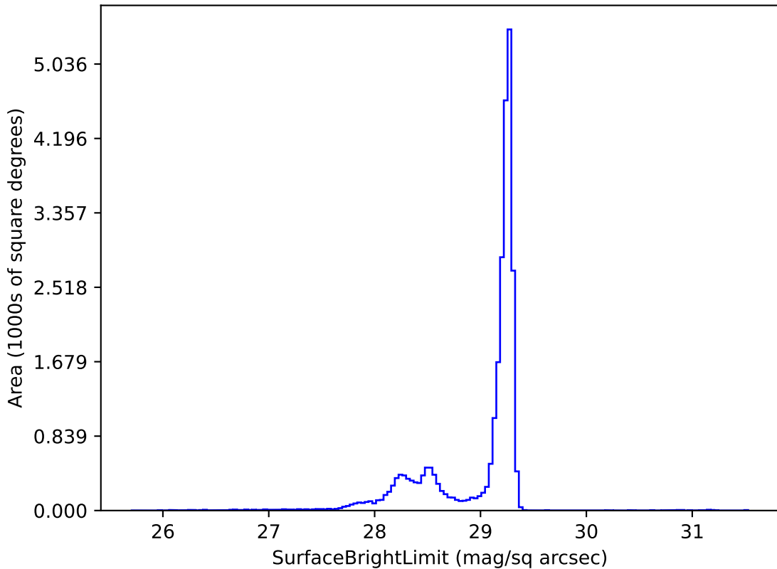
too_elab_r8_d3_griz_v3.4_10yrs z: SurfaceBrightLimit
