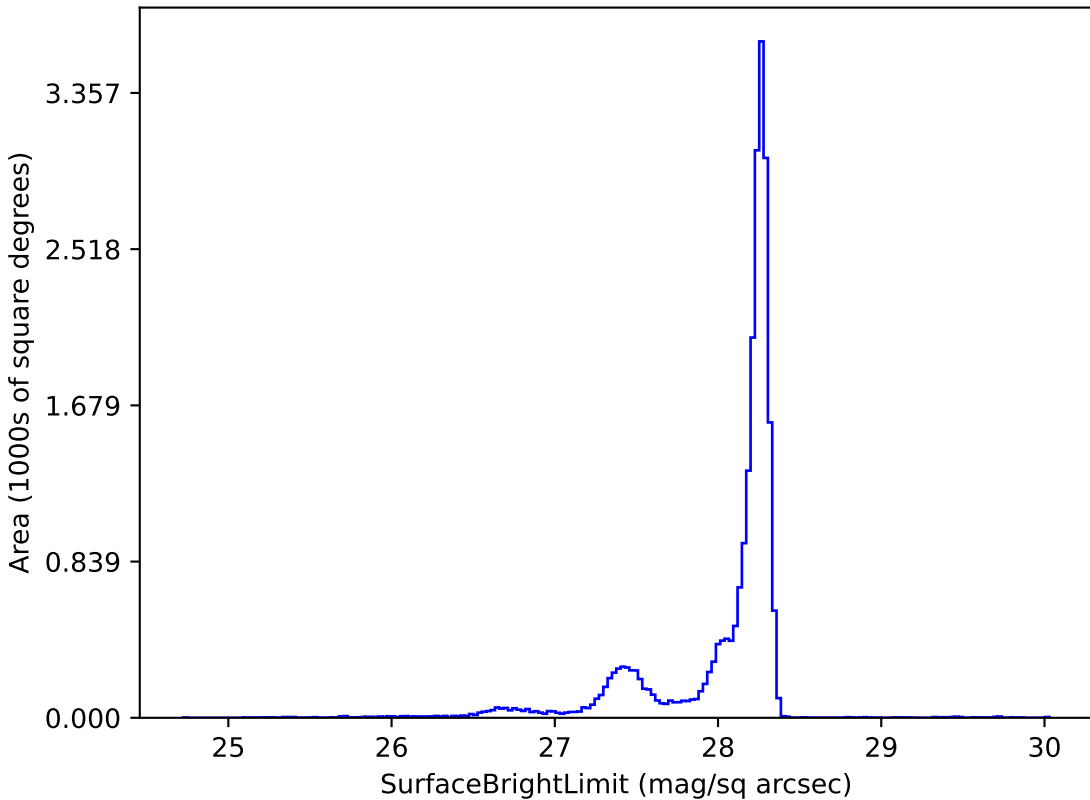
too_elab_r8_d3_griz_v3.4_10yrs y: SurfaceBrightLimit
