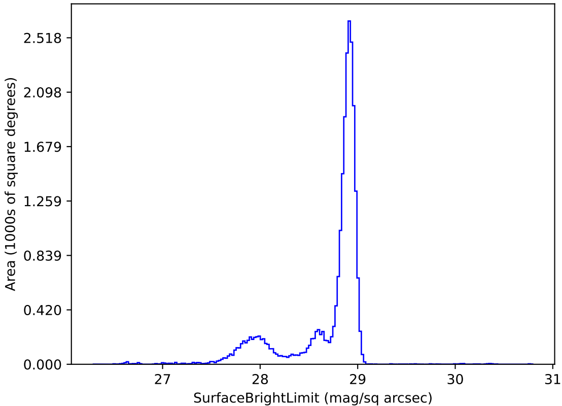
too_elab_r8_d3_griz_v3.4_10yrs u: SurfaceBrightLimit
