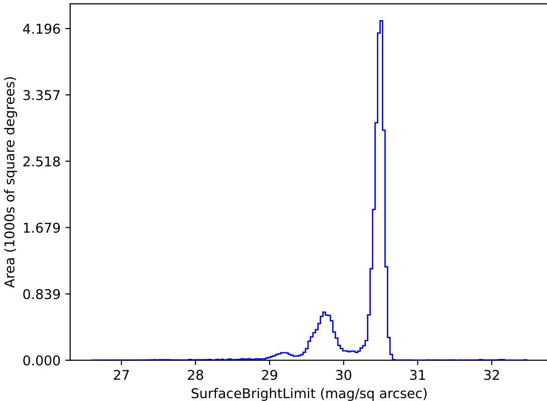
too_elab_r8_d3_griz_v3.4_10yrs r: SurfaceBrightLimit
