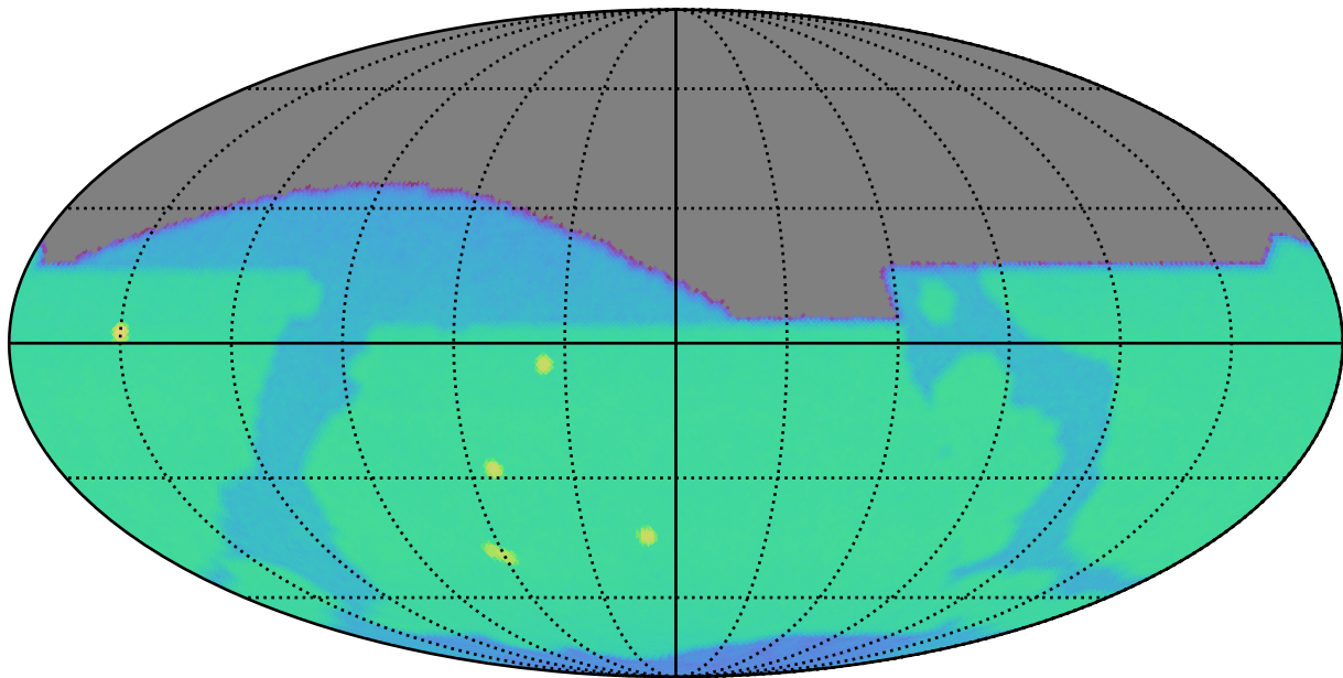
too_elab_r8_d3_griz_v3.4_10yrs i: SurfaceBrightLimit
