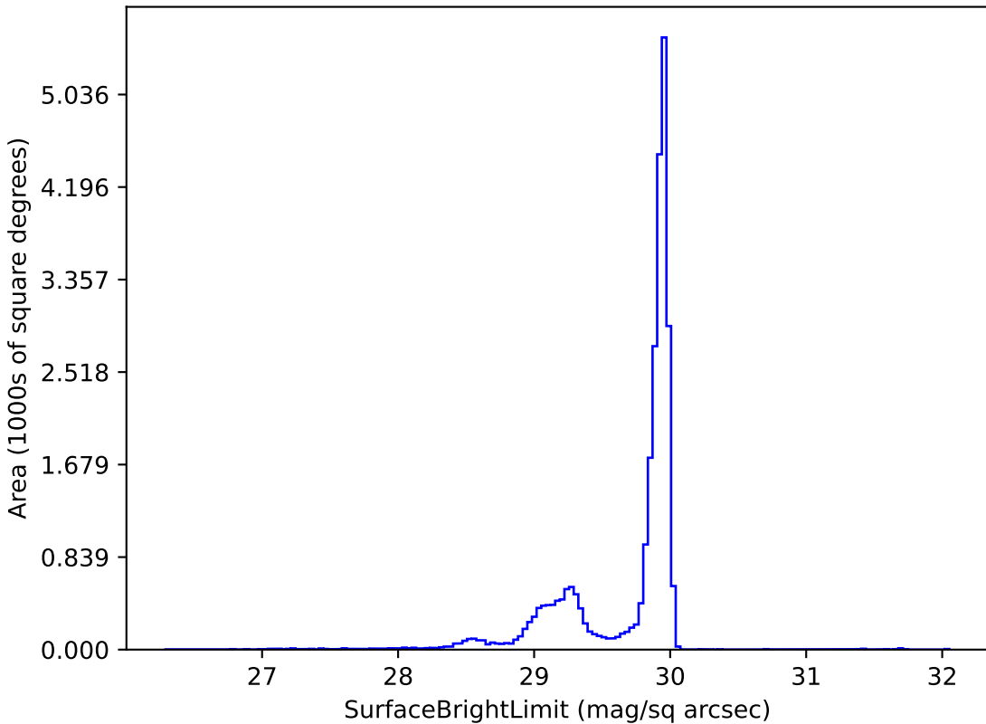
too_elab_r8_d3_griz_v3.4_10yrs i: SurfaceBrightLimit
