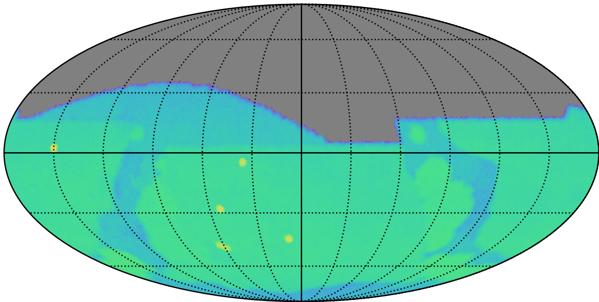
too_elab_r8_d3_griz_v3.4_10yrs g: SurfaceBrightLimit
