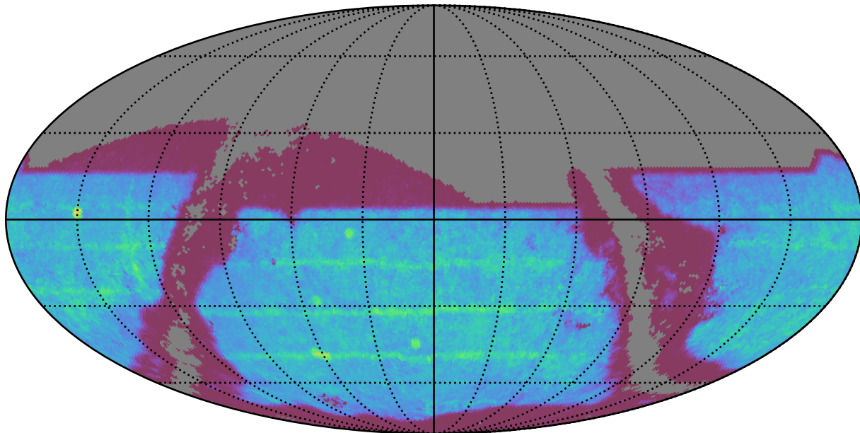
too_elab_r8_d3_griz_v3.4_10yrs : SNSLMetric
