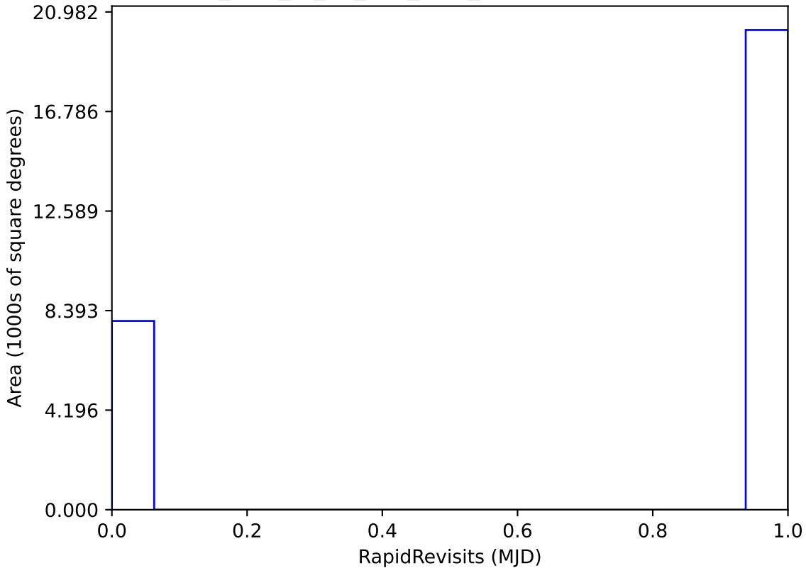
too_elab_r8_d3_griz_v3.4_10yrs : RapidRevisits
