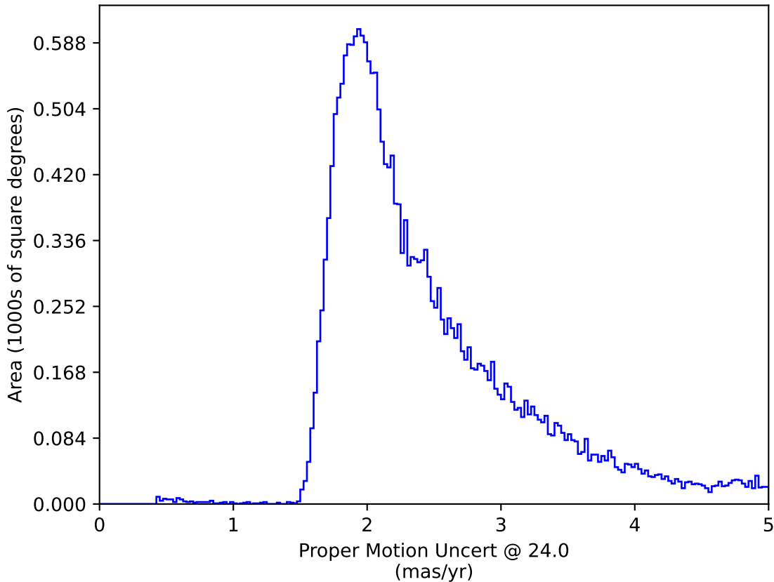
too_elab_r8_d3_griz_v3.4_10yrs : Proper Motion Uncert @ 24.0
