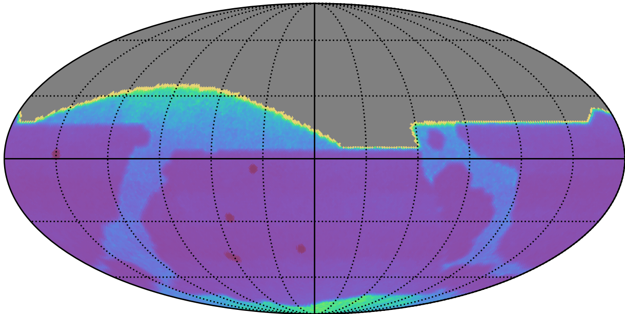
too_elab_r8_d3_griz_v3.4_10yrs : Proper Motion Uncert @ 20.5
