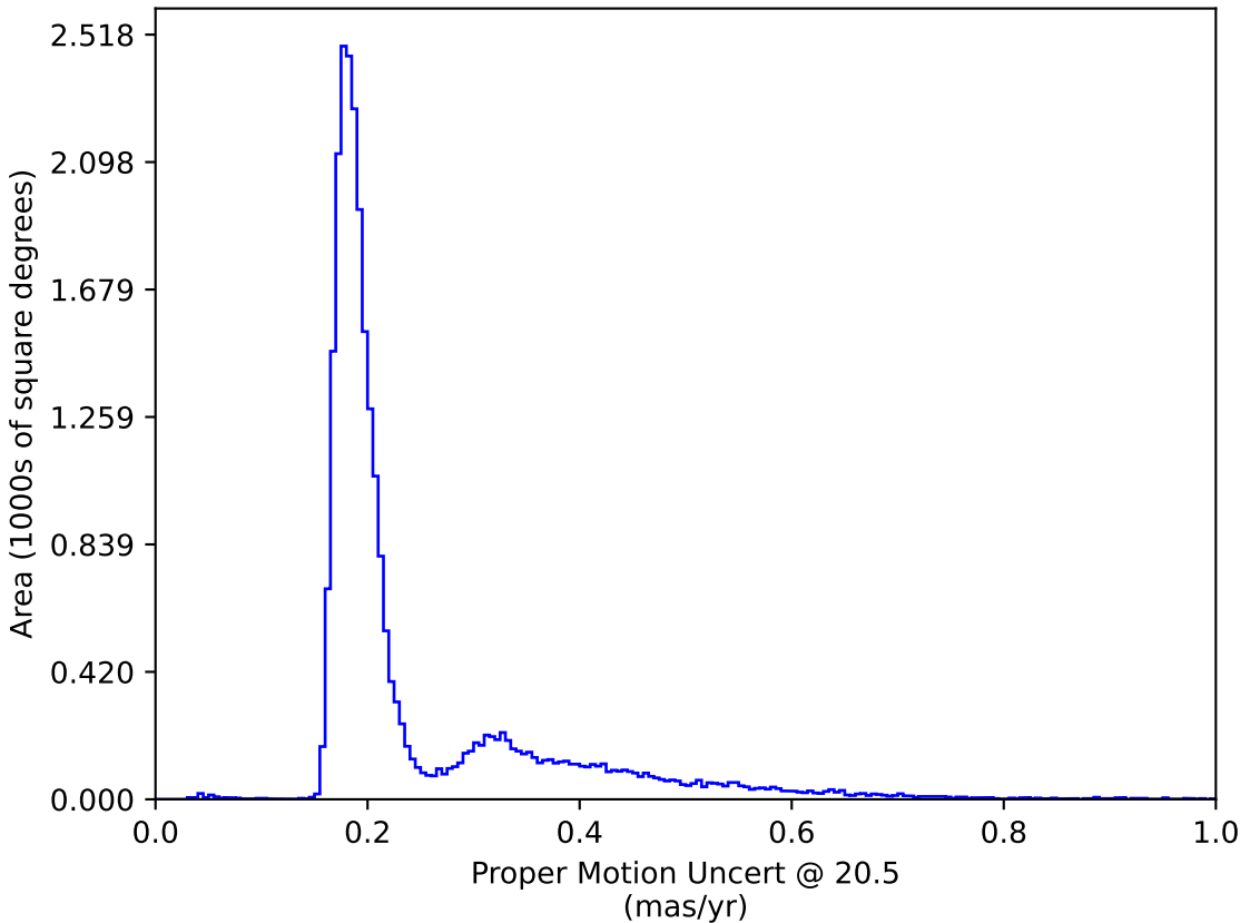
too_elab_r8_d3_griz_v3.4_10yrs : Proper Motion Uncert @ 20.5
