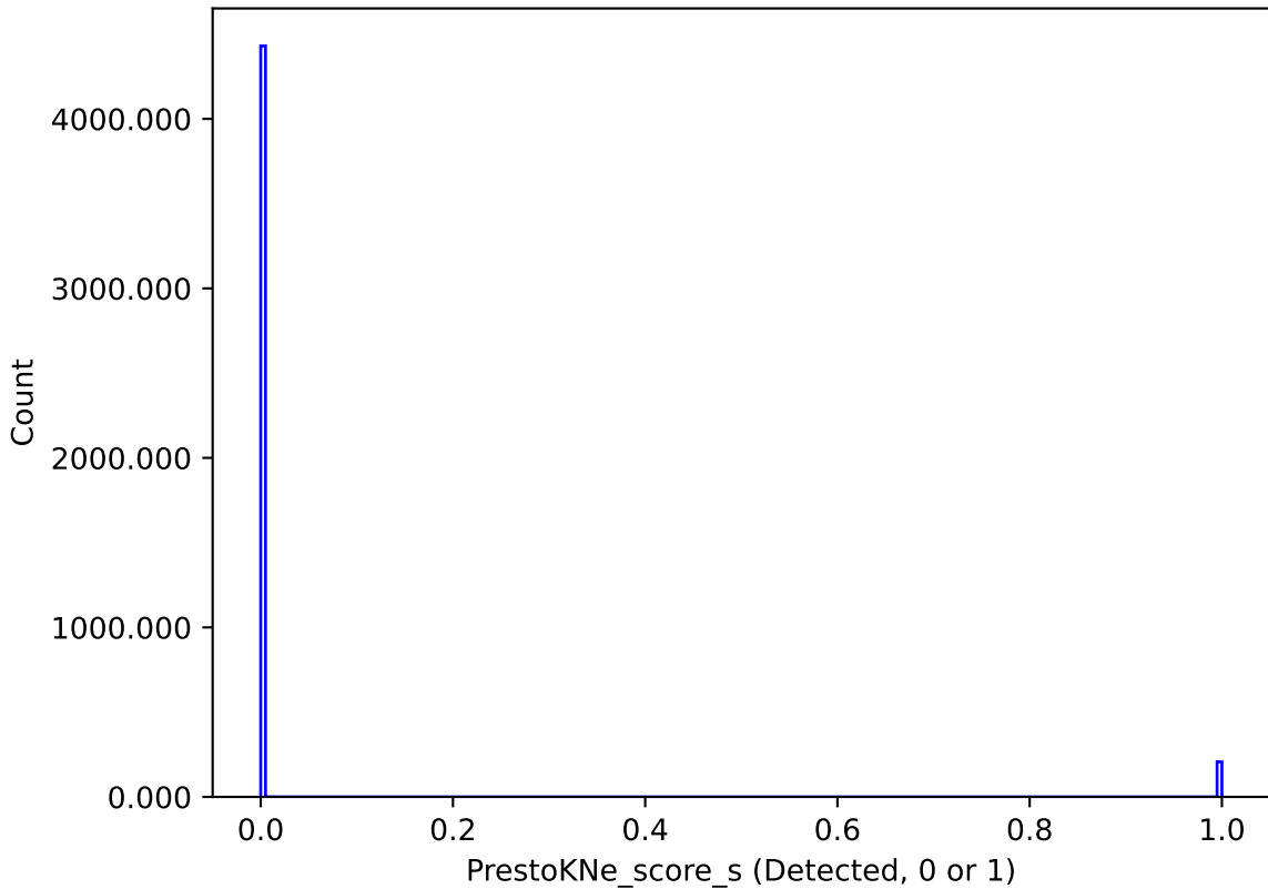
too_elab_r8_d3_griz_v3.4_10yrs : PrestoKNe_score_s
