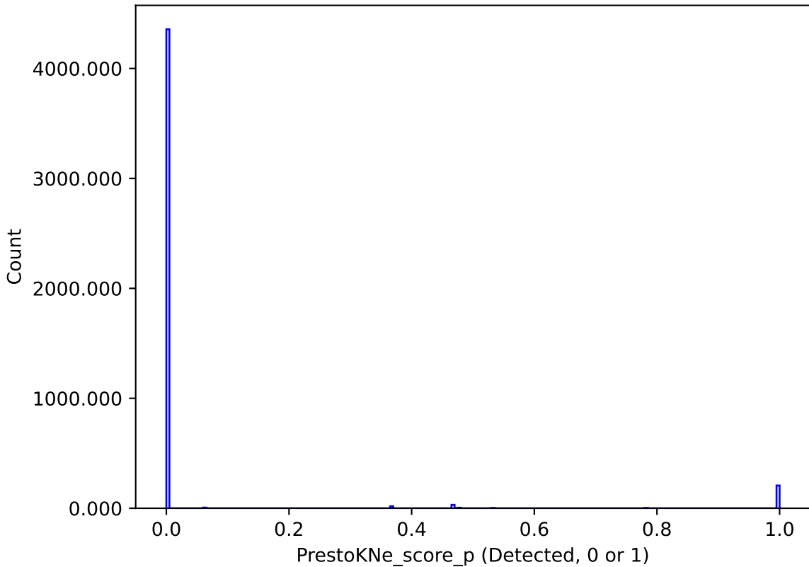
too_elab_r8_d3_griz_v3.4_10yrs : PrestoKNe_score_p
