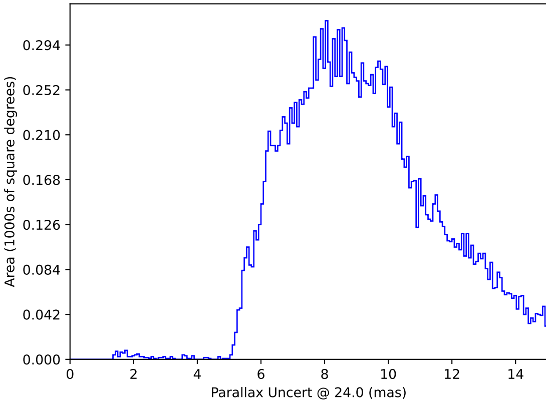
too_elab_r8_d3_griz_v3.4_10yrs : Parallax Uncert @ 24.0
