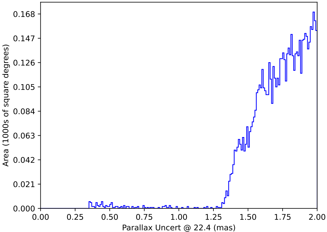
too_elab_r8_d3_griz_v3.4_10yrs : Parallax Uncert @ 22.4
