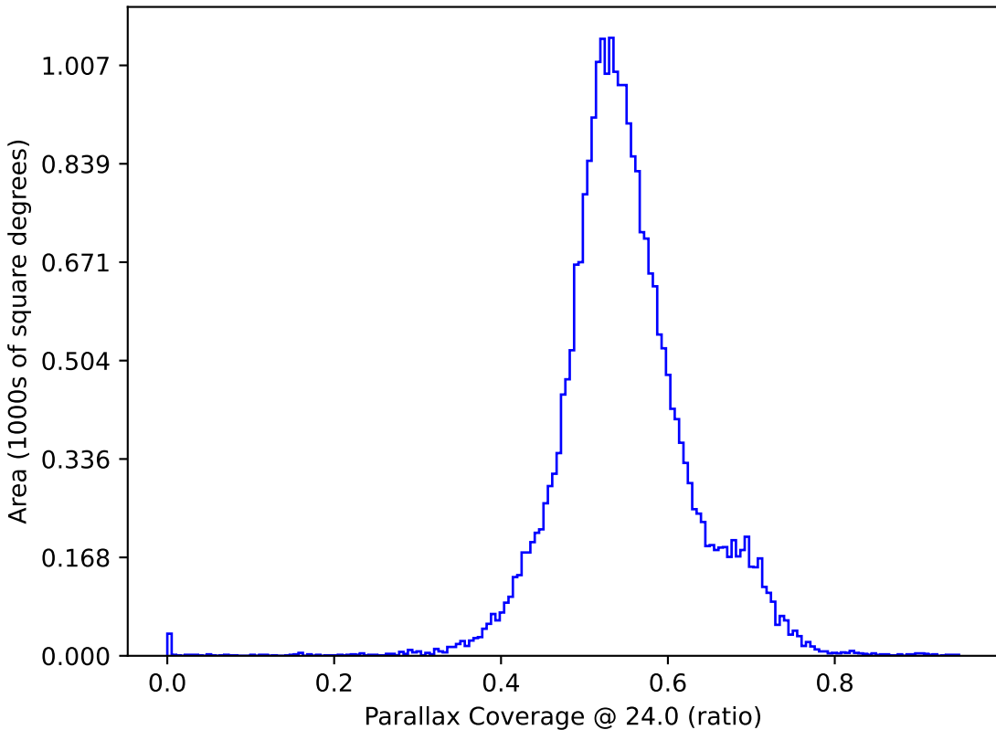
too_elab_r8_d3_griz_v3.4_10yrs : Parallax Coverage @ 24.0
