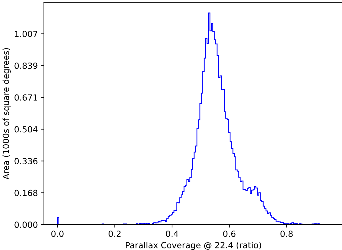
too_elab_r8_d3_griz_v3.4_10yrs : Parallax Coverage @ 22.4
