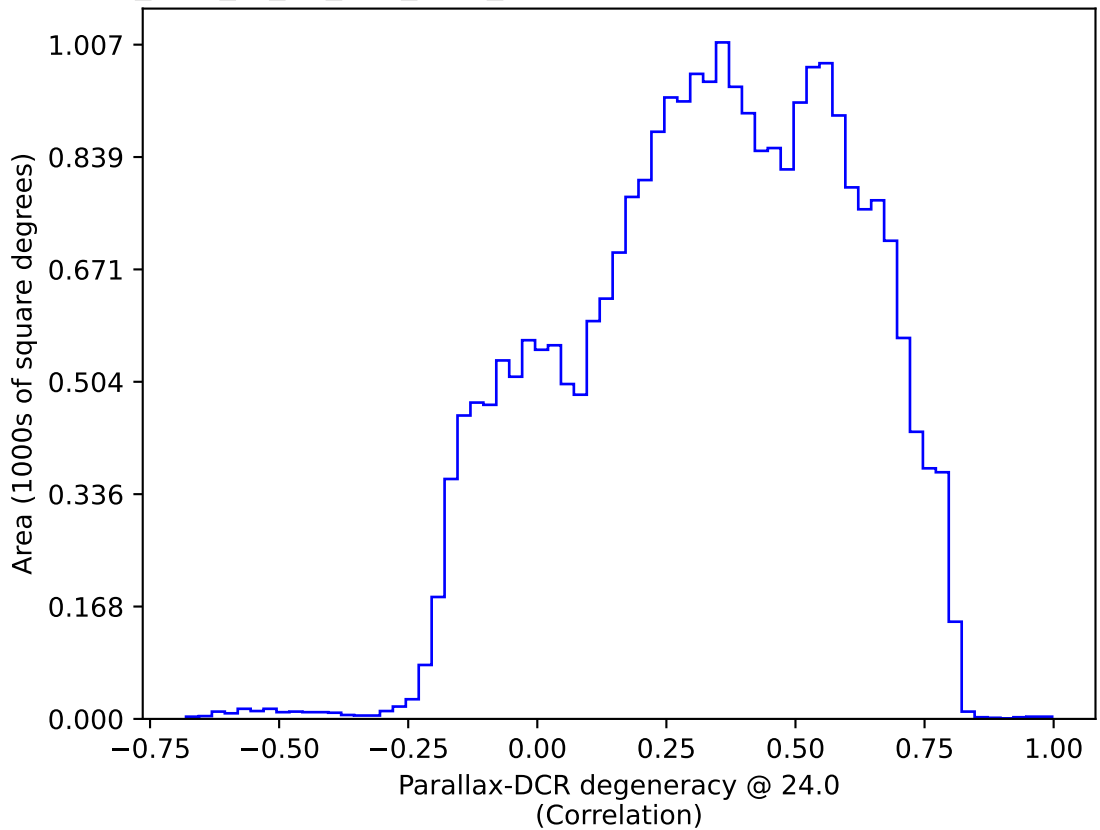
too_elab_r8_d3_griz_v3.4_10yrs : Parallax-DCR degeneracy @ 24.0
