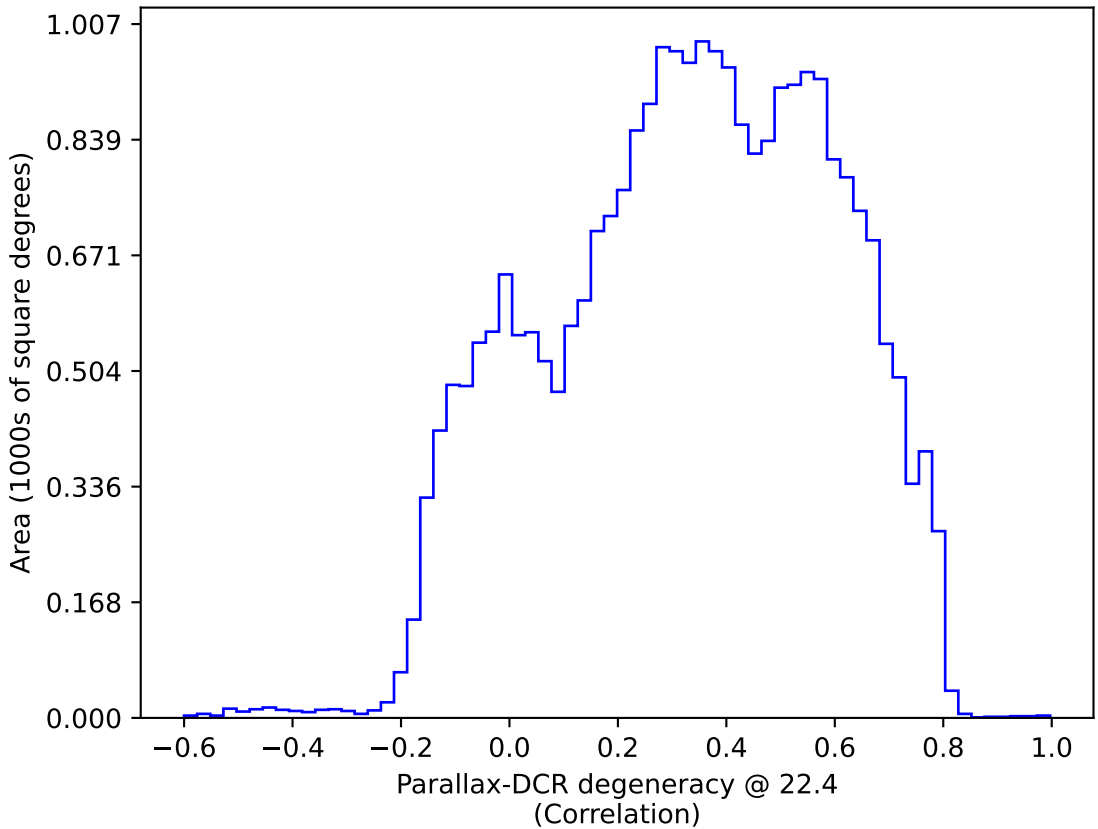
too_elab_r8_d3_griz_v3.4_10yrs : Parallax-DCR degeneracy @ 22.4
