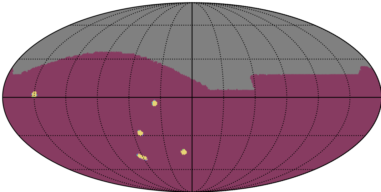
too_elab_r8_d3_griz_v3.4_10yrs : NumberOfQuickRevisits
