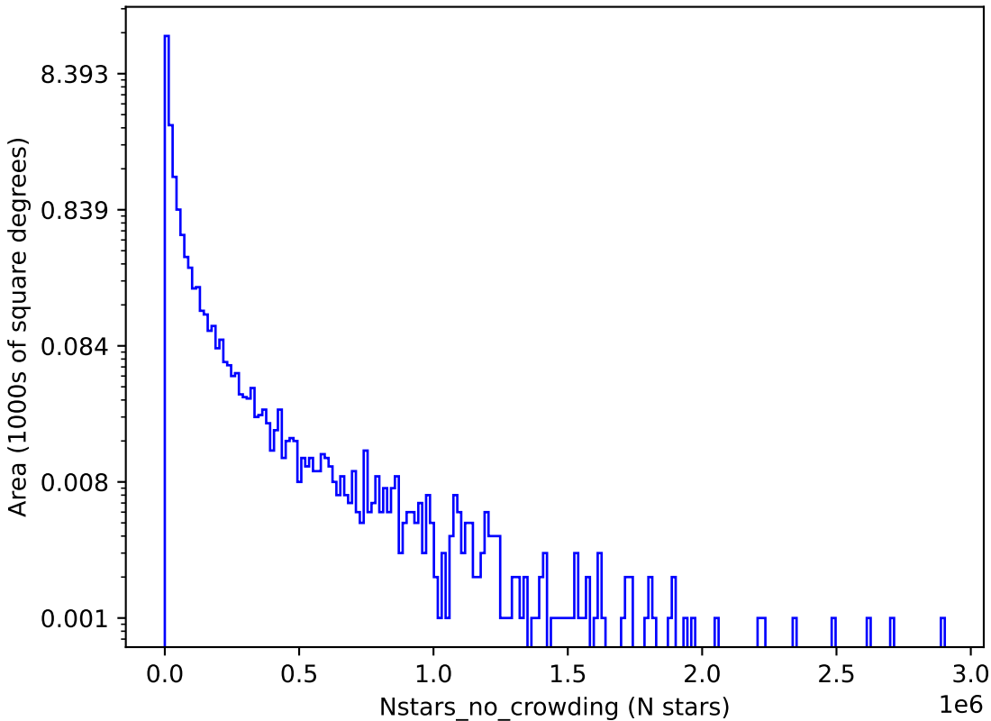
too_elab_r8_d3_griz_v3.4_10yrs u: Nstars_no_crowding
