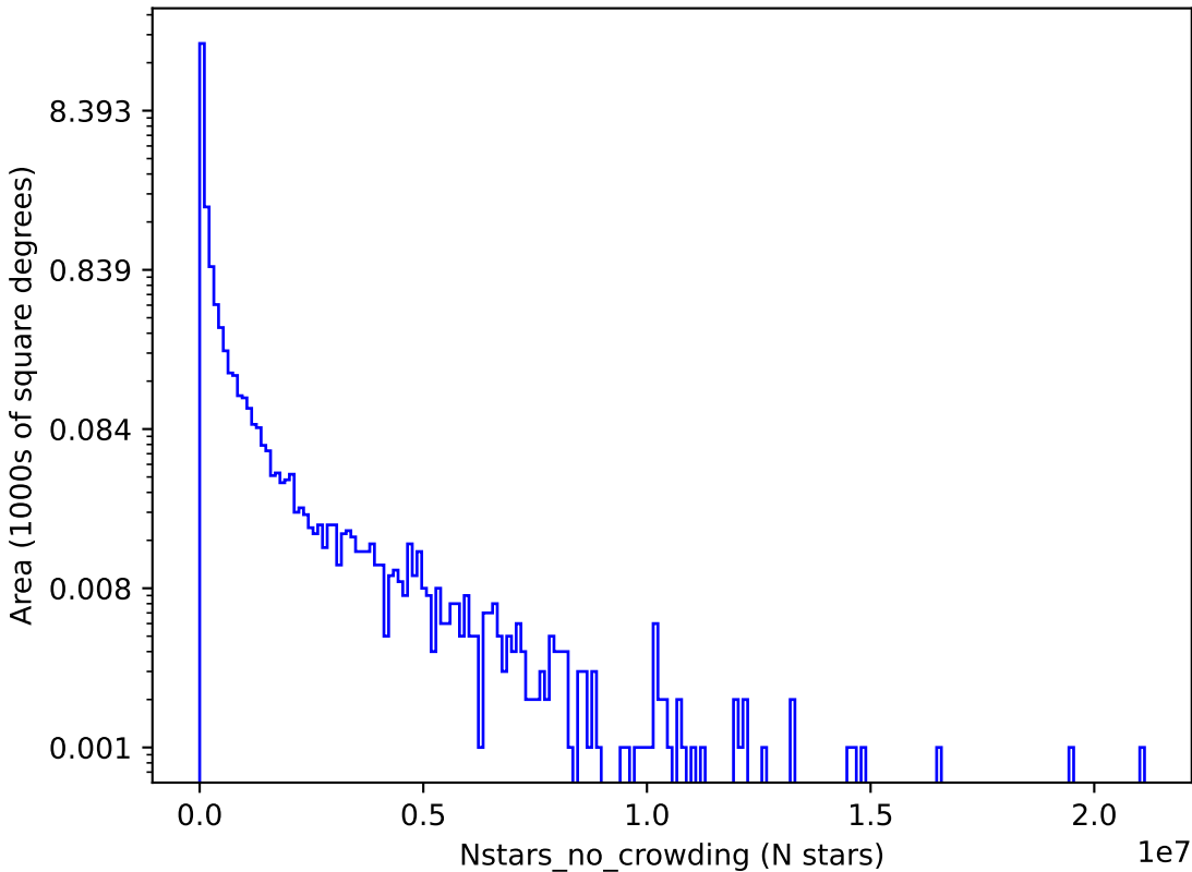
too_elab_r8_d3_griz_v3.4_10yrs r: Nstars_no_crowding
