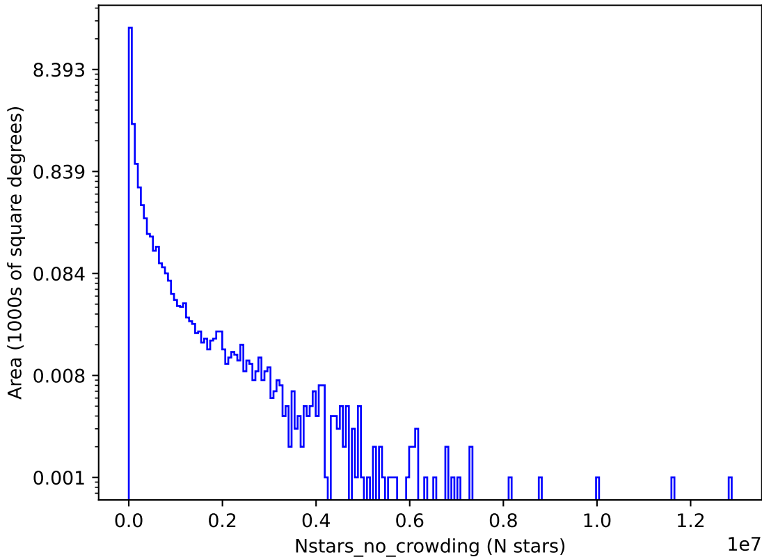
too_elab_r8_d3_griz_v3.4_10yrs g: Nstars_no_crowding
