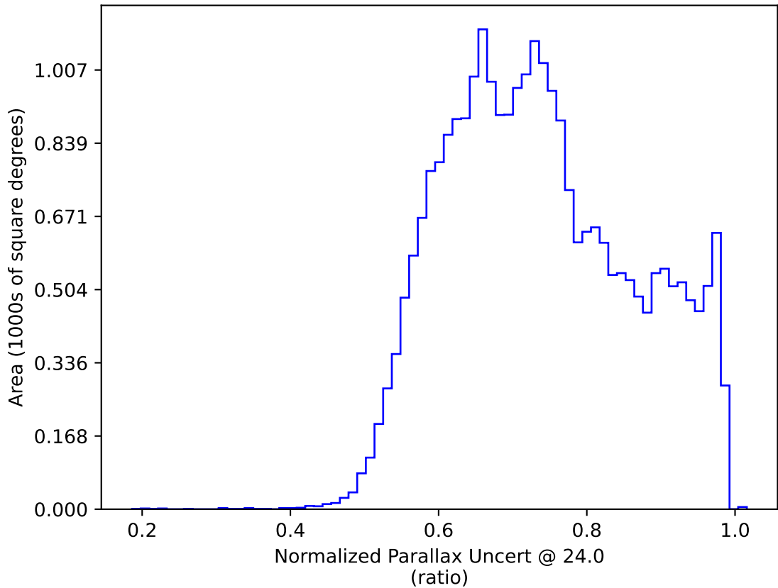
too_elab_r8_d3_griz_v3.4_10yrs : Normalized Parallax Uncert @ 24.0
