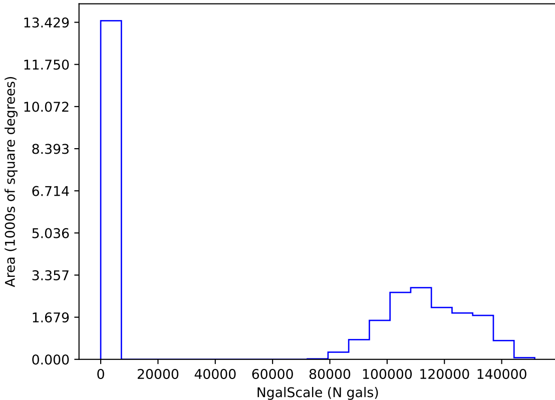
too_elab_r8_d3_griz_v3.4_10yrs i: NgalScale
