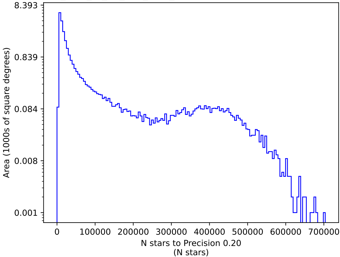
too_elab_r8_d3_griz_v3.4_10yrs z: N stars to Precision 0.20
