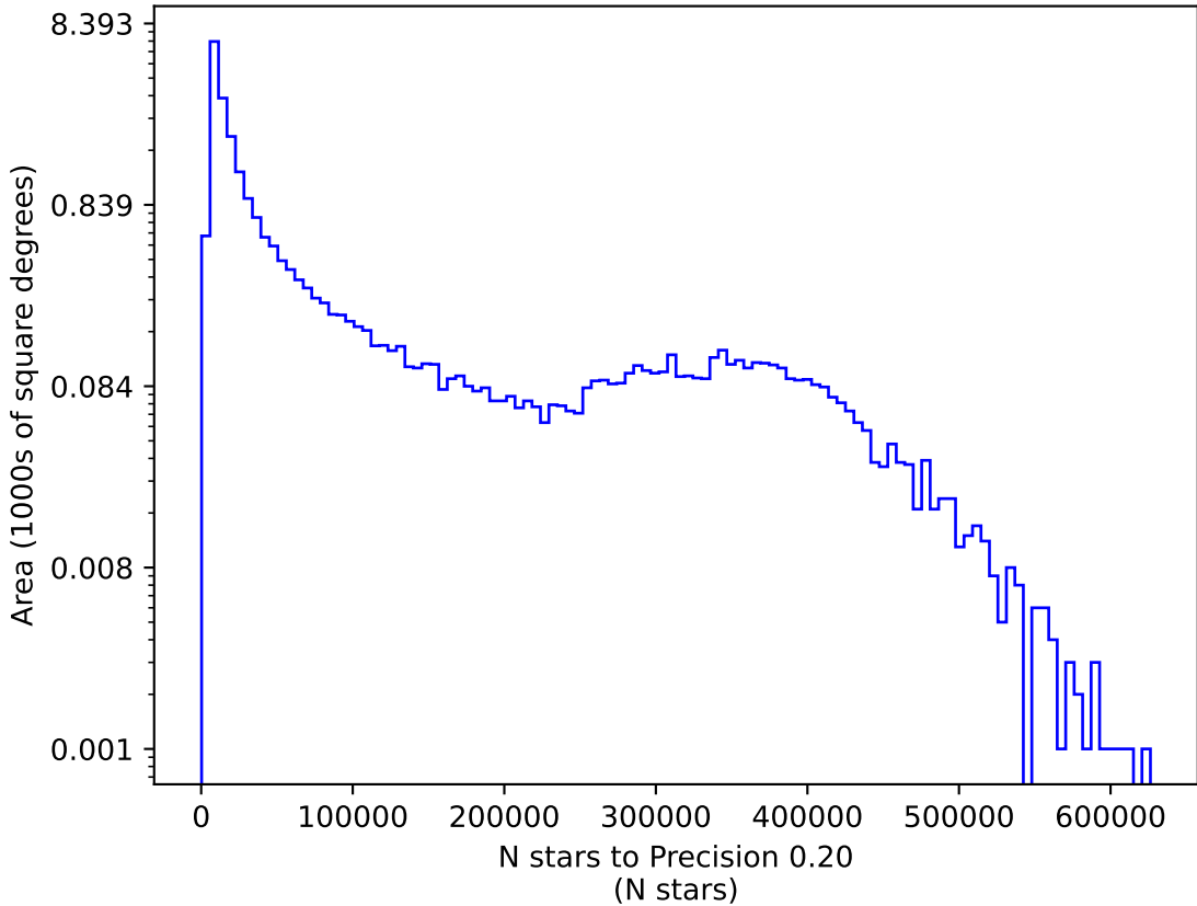
too_elab_r8_d3_griz_v3.4_10yrs y: N stars to Precision 0.20
