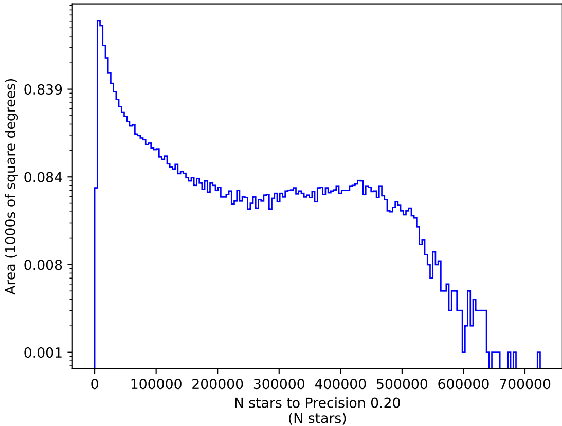
too_elab_r8_d3_griz_v3.4_10yrs r: N stars to Precision 0.20
