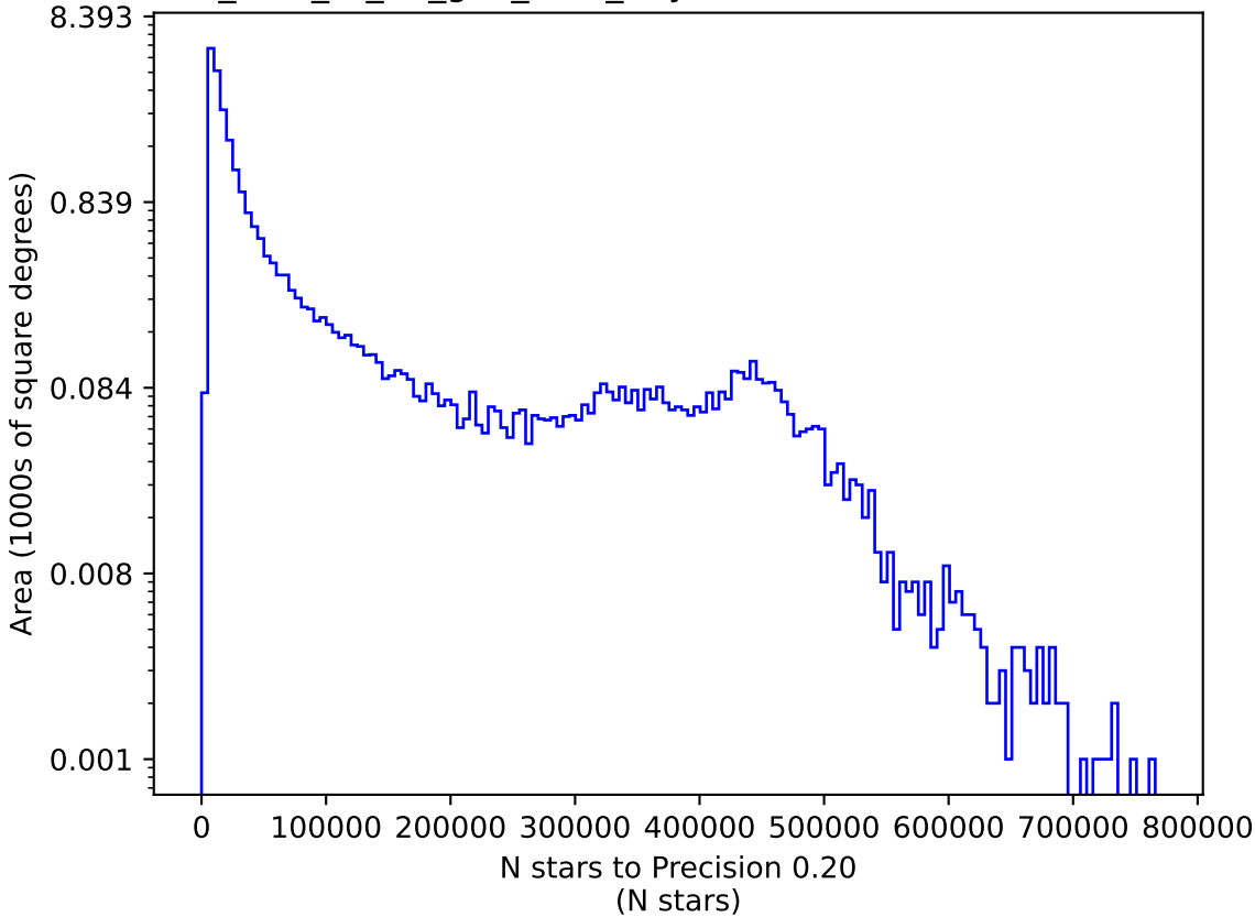
too_elab_r8_d3_griz_v3.4_10yrs i: N stars to Precision 0.20
