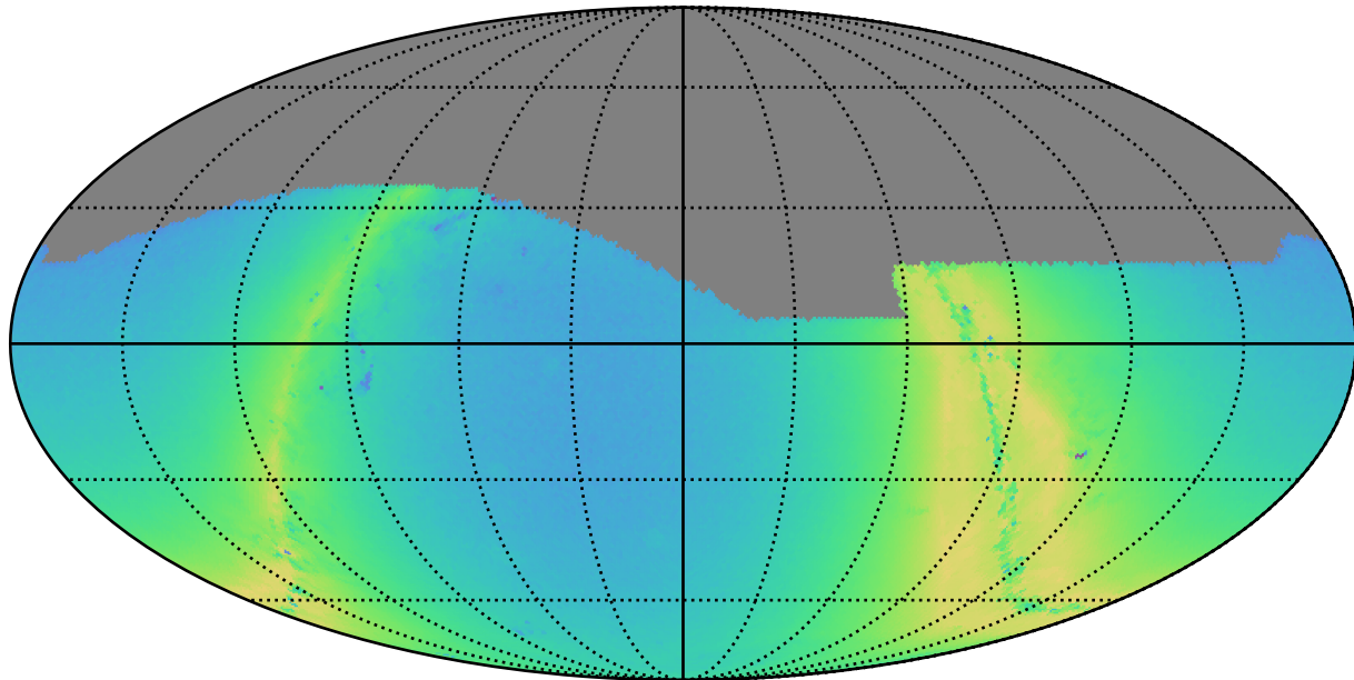
too_elab_r8_d3_griz_v3.4_10yrs g: N stars to Precision 0.20
