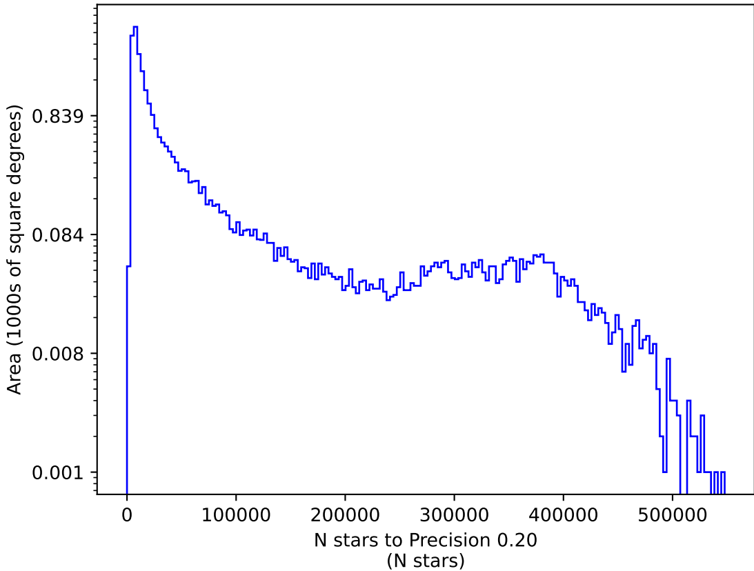
too_elab_r8_d3_griz_v3.4_10yrs g: N stars to Precision 0.20
