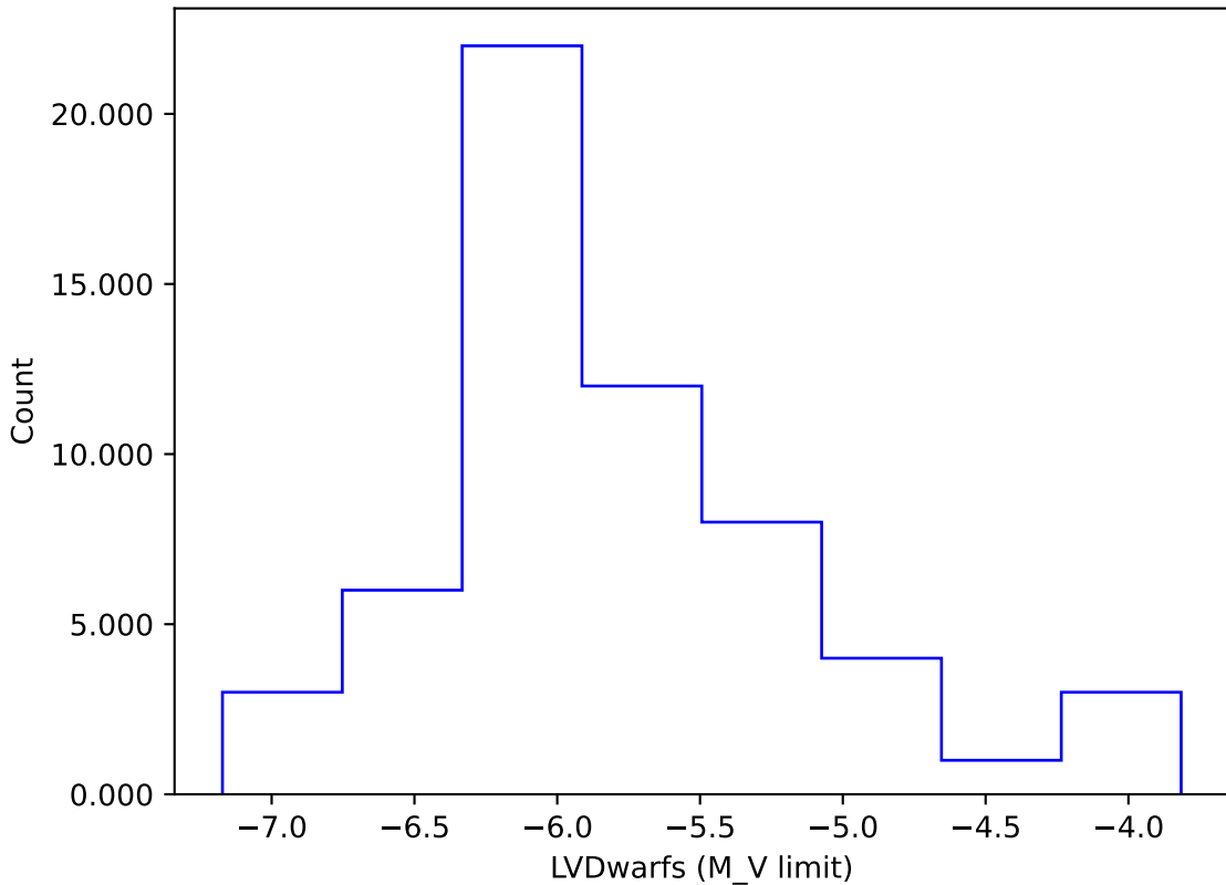
too_elab_r8_d3_griz_v3.4_10yrs gi: LVDwarfs
