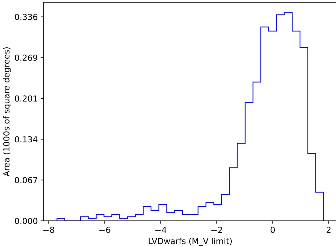
too_elab_r8_d3_griz_v3.4_10yrs gi SCP: LVDwarfs
