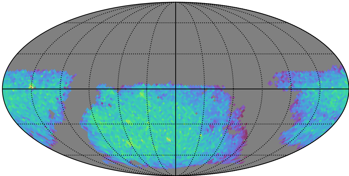
too_elab_r8_d3_griz_v3.4_10yrs gi: LVDwarfs
