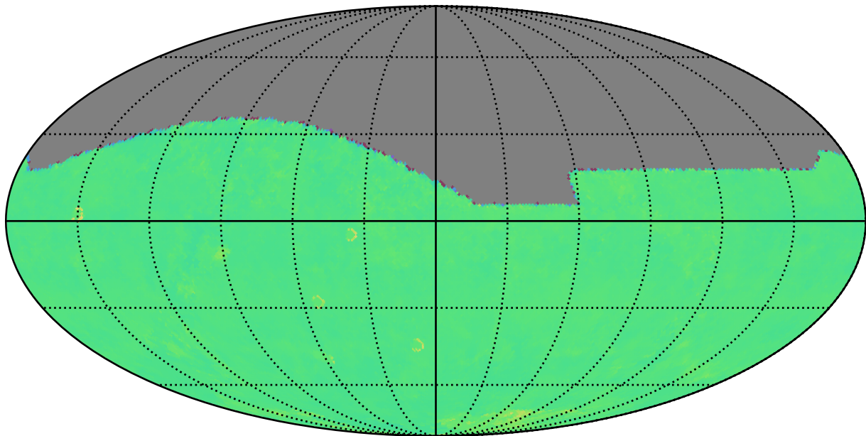
too_elab_r8_d3_griz_v3.4_10yrs r: Kuiper rotTelPos
