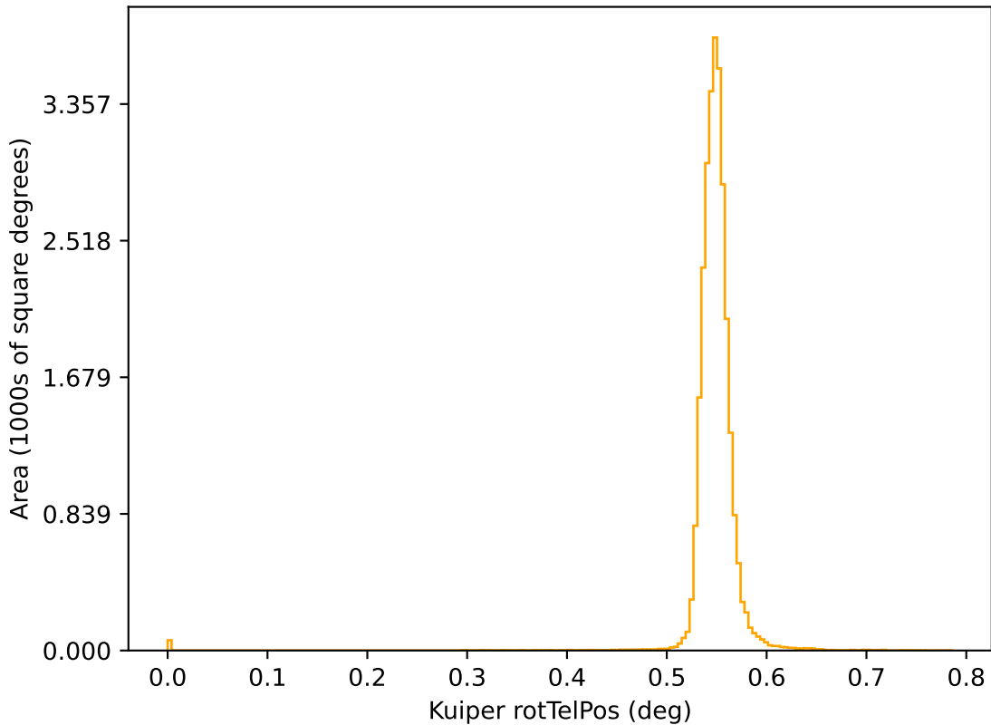
too_elab_r8_d3_griz_v3.4_10yrs r: Kuiper rotTelPos
