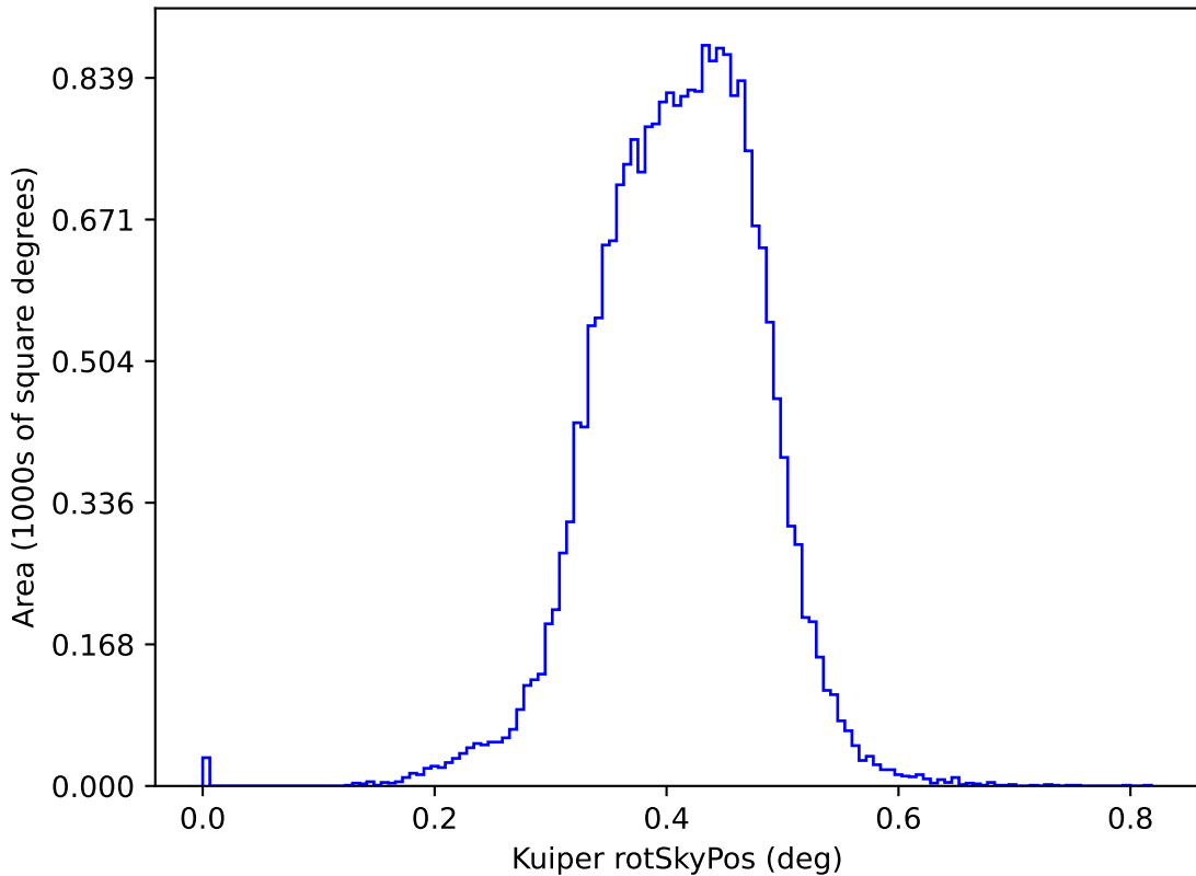
too_elab_r8_d3_griz_v3.4_10yrs y: Kuiper rotSkyPos
