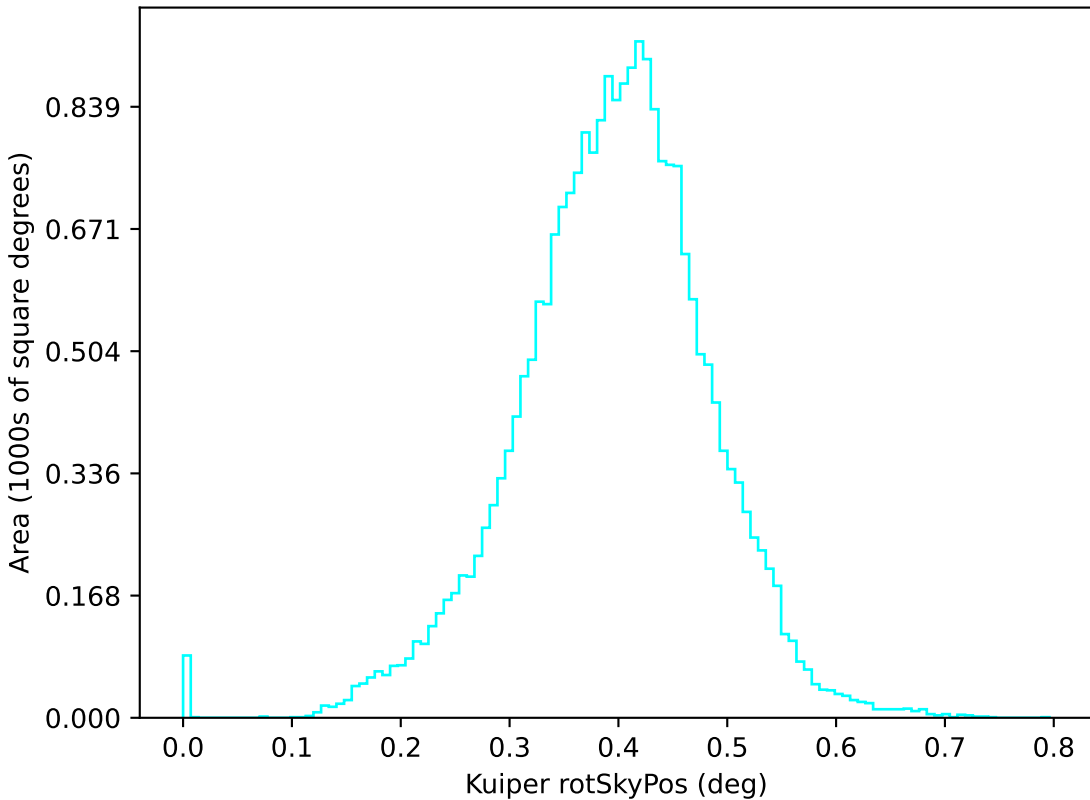
too_elab_r8_d3_griz_v3.4_10yrs u: Kuiper rotSkyPos
