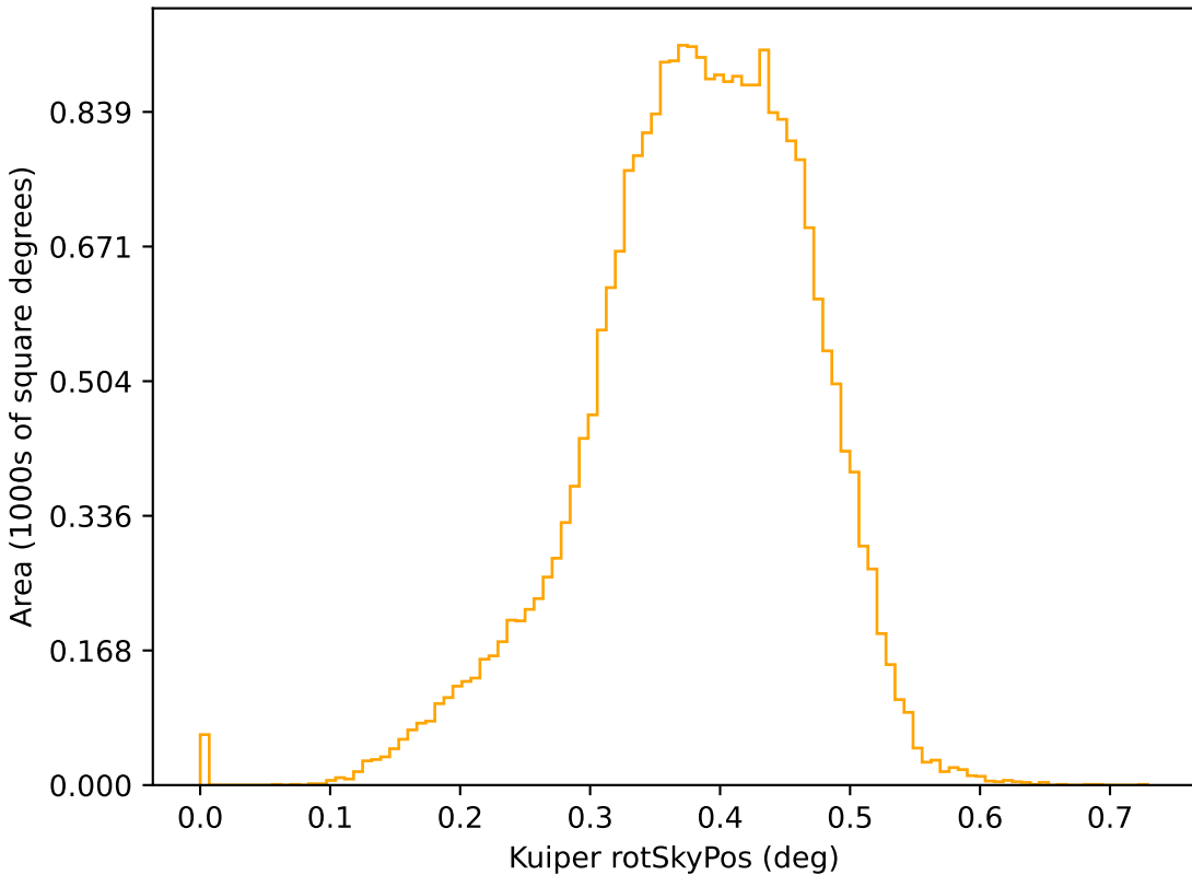
too_elab_r8_d3_griz_v3.4_10yrs r: Kuiper rotSkyPos
